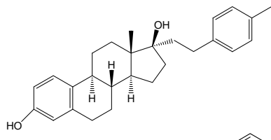
3-Hydroxy-17α-(4-methylbenzyl)estra-1,3,5(10)-trien-17β-ol
