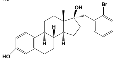
3-Hydroxy-17α-(2-bromobenzyl)estra-1,3,5(10)-trien-17β-ol
