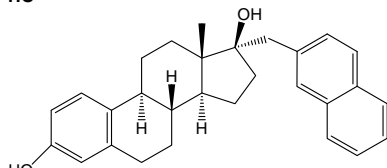
3-Hydroxy-17α-(2-Naphtylmethyl)estra-1,3,5(10)-trien-17β-ol
