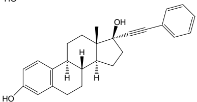
3-Hydroxy-17α-(2-phenylpropynyl)estra-1,3,5(10)-trien-17β-ol
