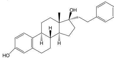
3-Hydroxy-17α-(2-phenylethyl)estra-1,3,5(10)-trien-17β-ol
