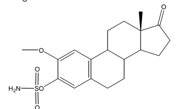
3-Hydroxy-2-methoxyestra-1(10),3,4-trien-17-one 3-sulfamate (2-Methoxyestrone sulfamate)
