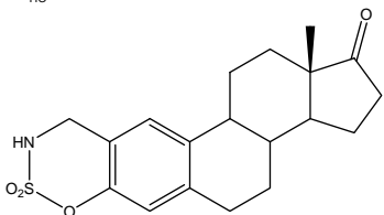
(13a S )-13a-methyl-(2,3,3a,3b,4,5,9,10,11b,12,13,13a)dodecahydronaphtho-1 H -cyclopenta[7,8]phenanthro[3,2- e ][1,2,3]oxathiazin-1-one-8,8-dioxide
