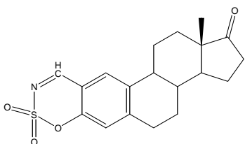
(13a S )-13a-methyl-(2,3,3a,3b,4,5,11b,12,13,13a)-decahydronaphtho-1 H -cyclopenta[7,8]phenanthro[3,2- e ][1,2,3]oxathiazin-1-one-8,8-dioxide
