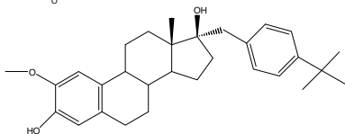
17 \alpha -(4- tert -butylbenzyl)-3-hydroxy-2-methoxyestra-1(10),3,4-trien-17 \beta -ol
