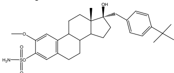
17 \alpha -(4- tert -butylbenzyl)-3-hydroxy-2-methoxyestra-1(10),3,4-trien-17 \beta -ol 3-sulfamate
